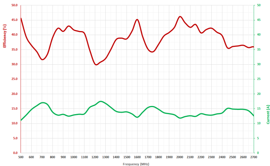
VM2K Current & Efficiency
