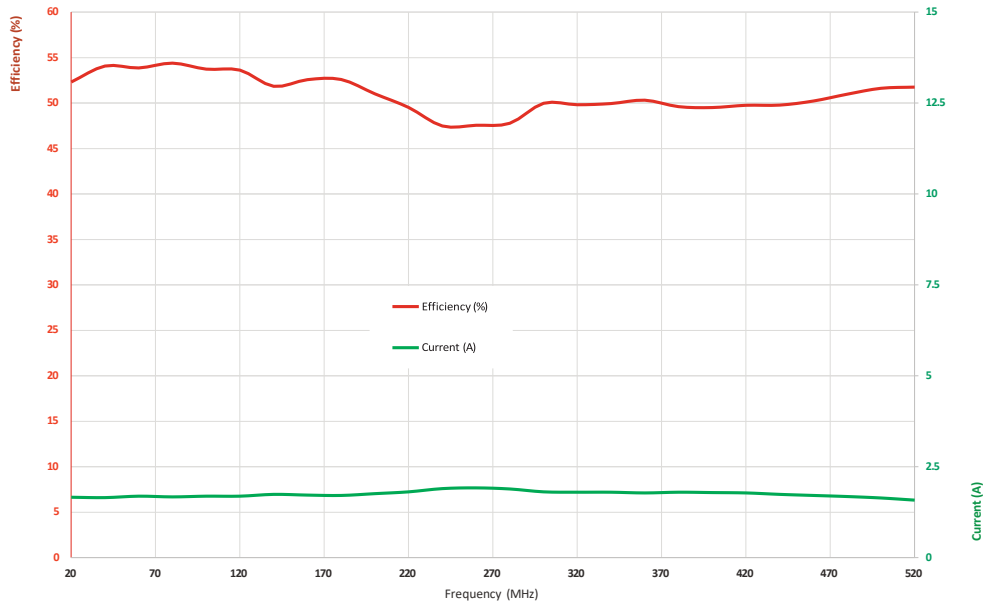
MP1BC2 Efficiency / Current
