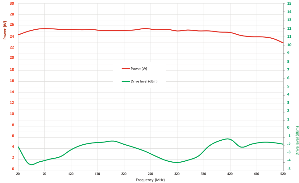
MP1BC2 Psat Power / Drive level
